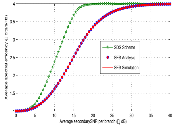
Fig. 5. Average spectral efficiency versus \overline{\gamma_s} (in dB).
