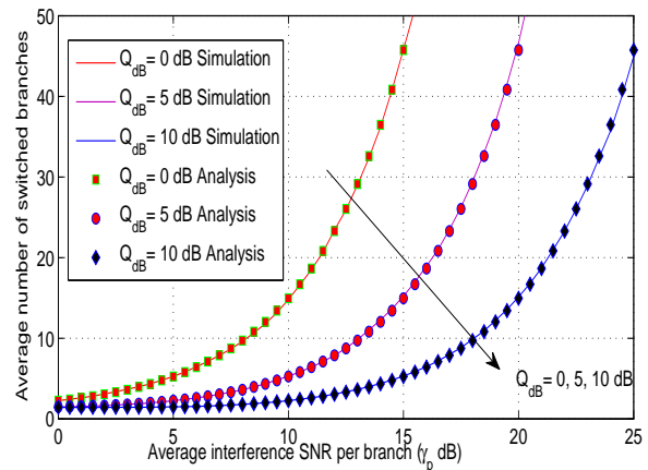
Fig. 4. Average number of switched branches versus \overline{\gamma_p} (in dB) for different levels of Q .
