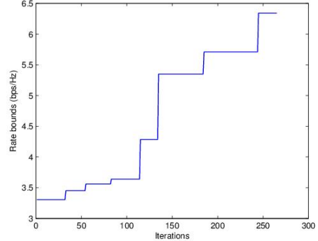
Fig. 3. Bounding progress of BB vs. the number of iterations
