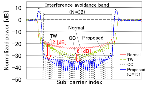
Figure 5. Power spectrum density of IA-PFT.
