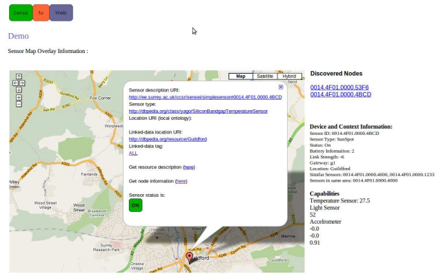
Figure 4: Sense2Web application
