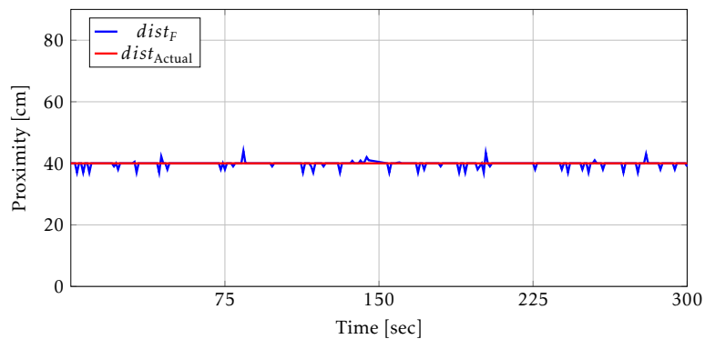
Figure 11. Proximity values ( dist_F and dist_{Actual} ) vs time
