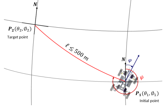
Figure 6. Navigational geometry of the robot in the geographic coordinate system
