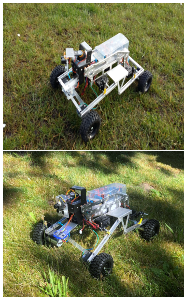
Figure 9. Performance evaluations in field tests
