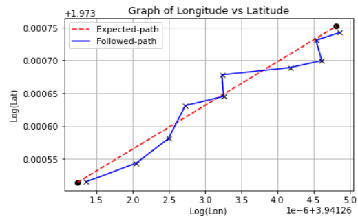
Figure 13. Path-plot 2: Graph visualizing the robot's routes (navigated distance \approx 120.78 m, number of obstacles = 5)
