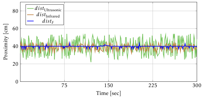
Figure 10. Proximity values (i.e., dist_{Ultrasonic} , dist_{Infrared} , and dist_F ) vs time
