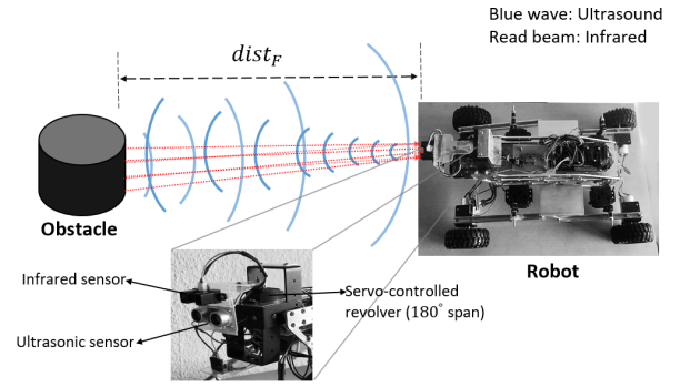
Figure 4. Depiction of obstacle's proximity measurement using both the ultrasonic and infrared sensor (Note: dist_F is the proximity of obstacle from the robot)
