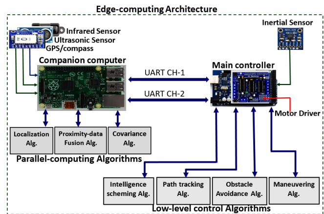
Figure 3. Edge-computing architecture, hardware, and algorithmic structure
