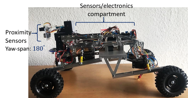
Figure 1. Experimental platform
