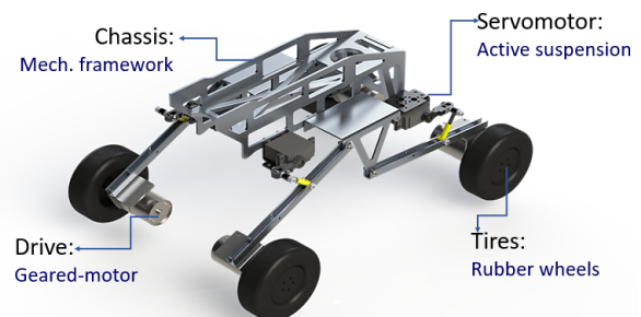
Figure 2. 3D model of robot mechanical system
