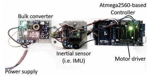
Figure 7. Configuration of the low-level controller (featuring the power supply, inertial sensor, main controller, motor driver, and their electrical connections)
