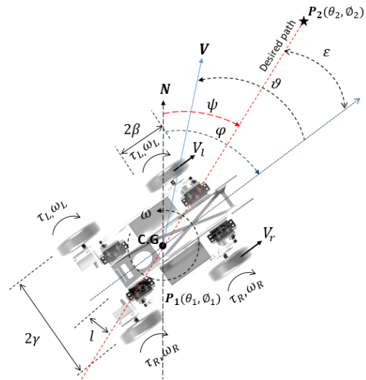
Figure 5. Robot navigation control model (Note: \theta_1 and \phi_1 are the latitude and longitude of P_1 , while \theta_2 and \phi_2 are those of P_2 , respectively)
