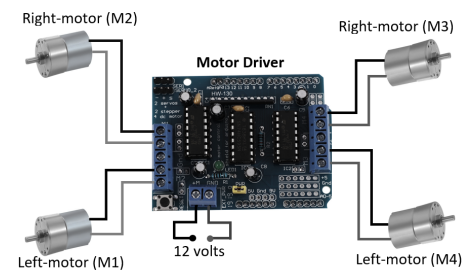
Figure 8. Connection of motors to the motor driver (the motor driver enables the main controller to control the speed and direction of the motors)
