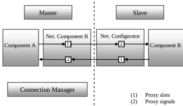
Figure 6. Remote connection between components in ARCS (Master-Slave)
