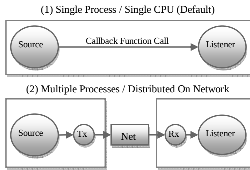
Figure 3. Tinmith transparent network distribution
