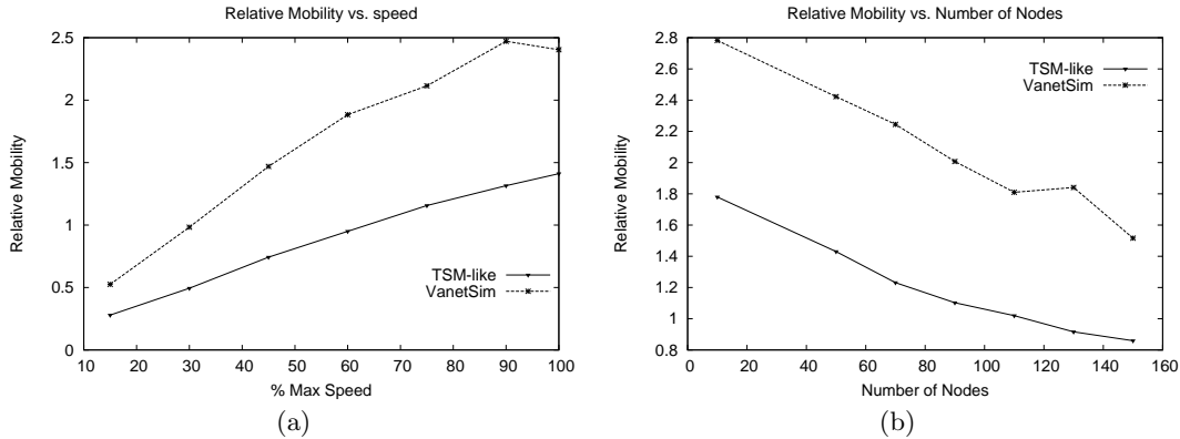
Figure 1: Relative Mobility
