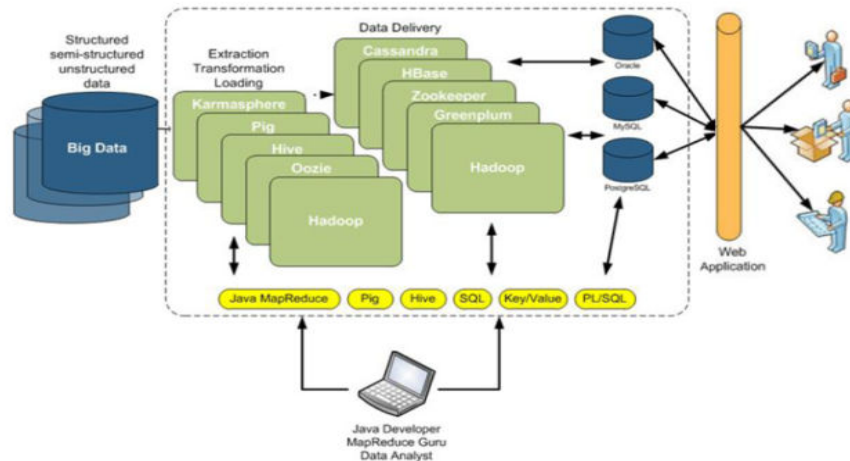
Fig 2. Hadoop Platform
