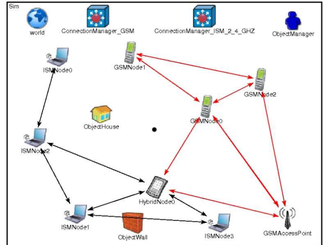
Figure 2: Illustration of a MiXiM Simulation
