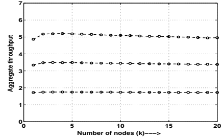
Figure 1: Total throughput (in Mbps) vs. number of users for radios using CSMA/CA random access, as standardised in IEEE 802.11, when all radios use the same physical transmission rate: 11 Mbps (top), 5.5 Mbps (middle), or 2 Mbps. The queues of the transmitters are saturated. This is an example of the function \bar{R}^c(k) for a network strategy that yields FSR.
