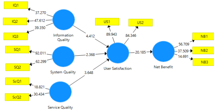
Fig. 4. Structural Model Results
