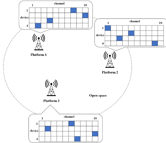
Fig. 1. System model
