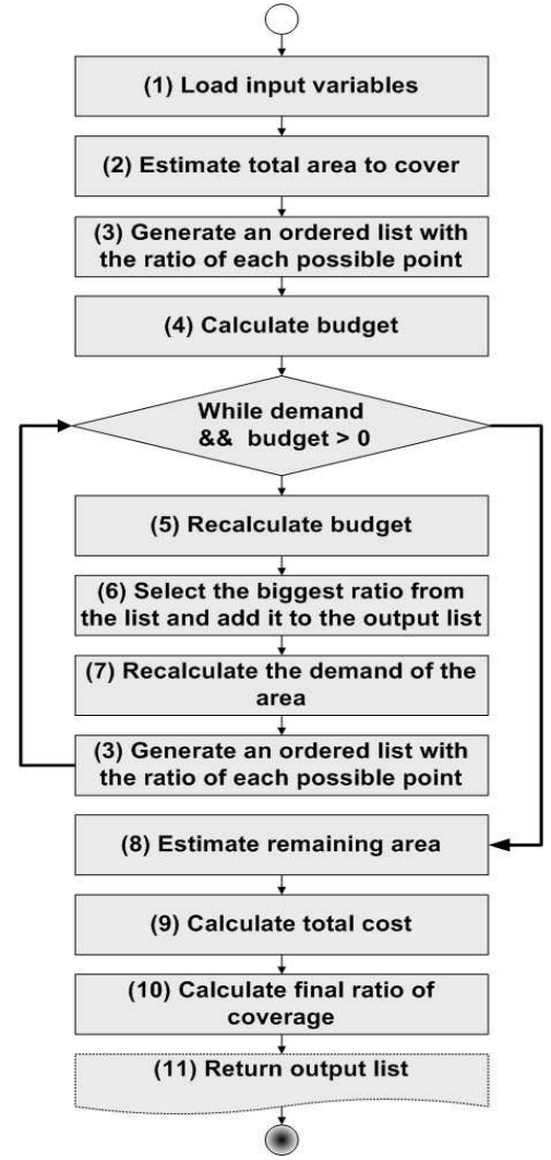
Figure 2: Flow chart
