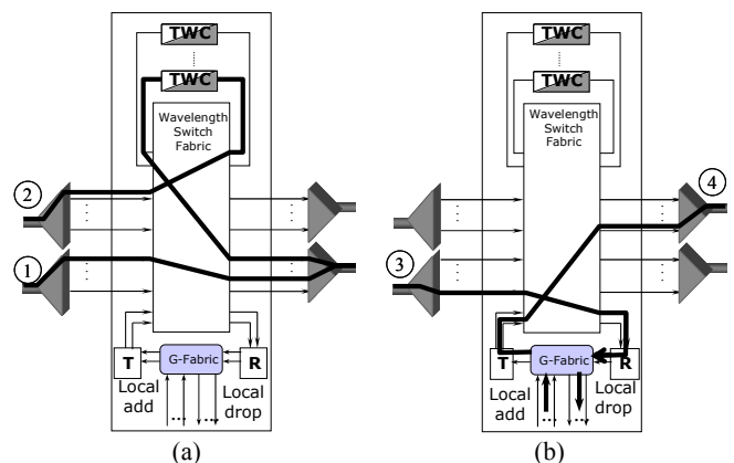
Figure 1. Functional blocks in the switching node.
