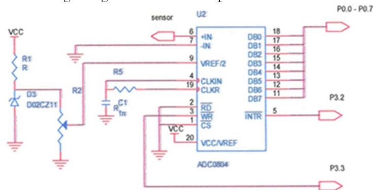
Figure 4. ADC 0804 schematic diagram
