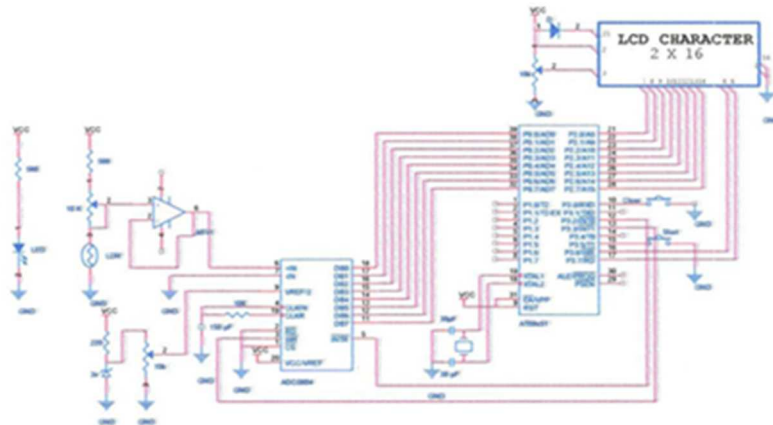
Figure 5. Overall system schematic
