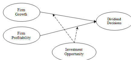
Fig.3. Theoretical Framework
