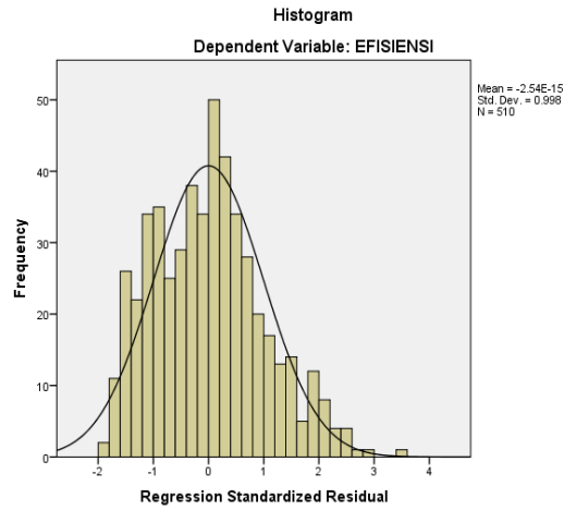
Fig.1. Normality Results using a Histogram chart
