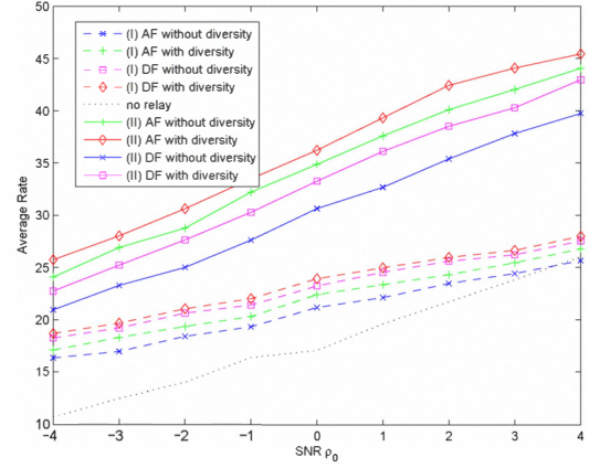
Fig. 4. Average Rate vs. SNR \rho_0 for two problems with four relay schemes and no relay schemes; M = 8 , K = 3 , N = 16 , r_2 = 500\text{m}
