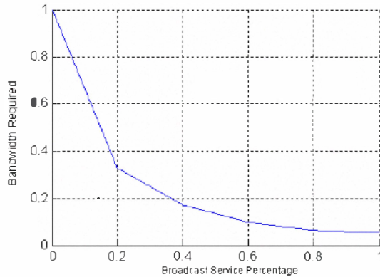
Fig. 6. Required Bandwidth vs. Broadcast Service Percentage
