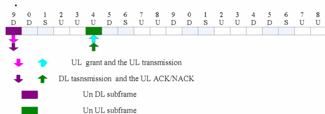
Figure 10. UL subframe allocation DL-UL Config #6
