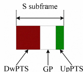
Figure 3. Structure of S subframe in TDD LTE[5].
