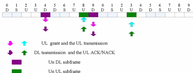
Figure 5. Un subframe allocation for DL-UL Config #1
