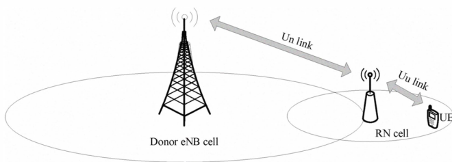
Figure 1. Backhaul (Un) link and access (Uu) link in a two-hop relay.
