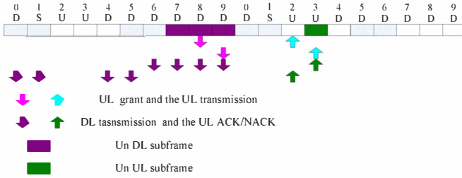
Figure 8. Un subframe allocation for DL-UL Config #4
