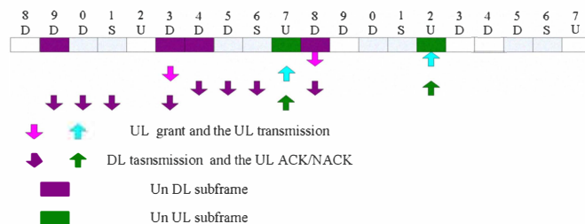
Figure 6. Un subframe allocation for DL-UL Config #2
