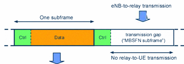
Figure 2. MBSFN and normal subframes for relay-UE link.
