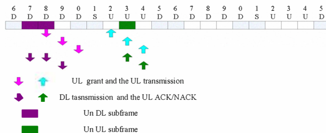
Figure 7. Un subframe allocation for DL-UL Config #3
