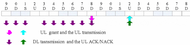
Figure 9. Un subframe allocation for DL-UL Config #5
