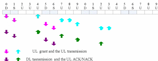
Figure 4. Un subframe allocation for DL-UL Config #0
