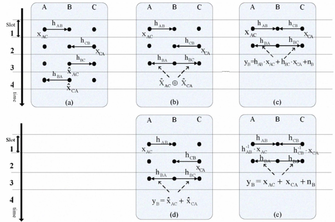
Fig. 1: (a) Conventional bi-directional relaying (b) Conventional DF BAT relaying (c) Conventional AF BAT relaying (d) EDF BAT relaying (e) PAF BAT relaying
