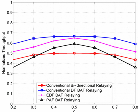
Fig. 3: Normalized throughput versus the distance between A-B, \sigma_A^2 = \sigma_B^2 = \sigma_C^2 = 0.2
