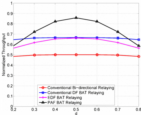
Fig. 4: Normalized throughput versus the distance between A-B, \sigma_A^2 = \sigma_B^2 = \sigma_C^2 = 0.15
