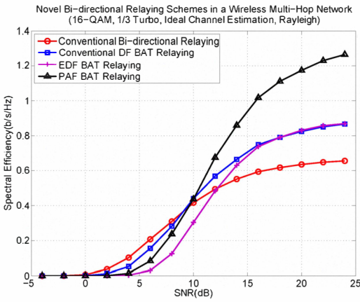
Fig. 6: Spectral Efficiency vs. SNR for Bi-directional Relaying Schemes
