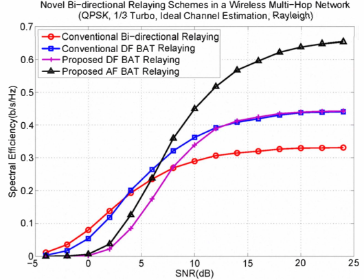
Fig. 5: Spectral Efficiency vs. SNR for Bi-directional Relaying Schemes
