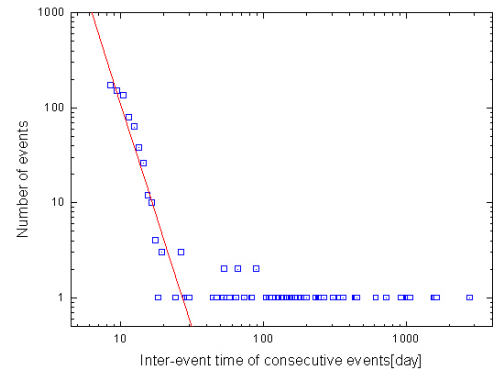
(a) simulation results of 2,000 executions based on the habit model
