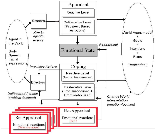
Figure 2. The FATiMA agent architecture.
