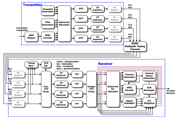
Fig. 1. Proposed 4x4 downlink transceiver.
