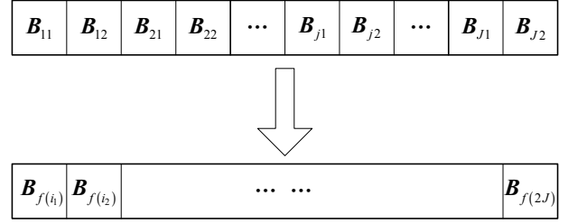
Fig. 4. Interleaving for signals, where the signals in different constellations are permuted together.
