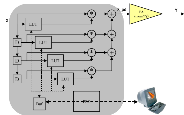
Figure 4. Structure of offline predistortion System
