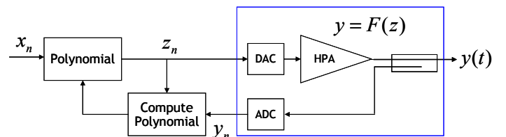
Figure 1. Polynomial predistorter
