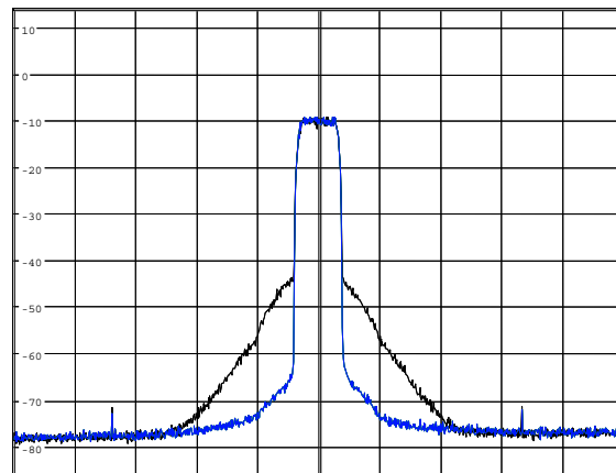
Figure 5. Spectrum of PA output for one carrier UMTS signal with and without DPD
