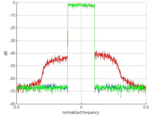
Figure 2. Power spectra
