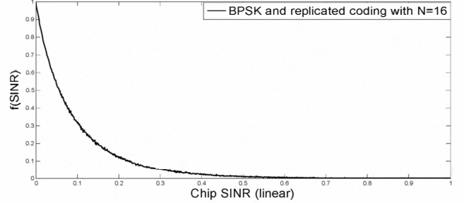
Fig. 1. f(\gamma) vs. chip level SINR
