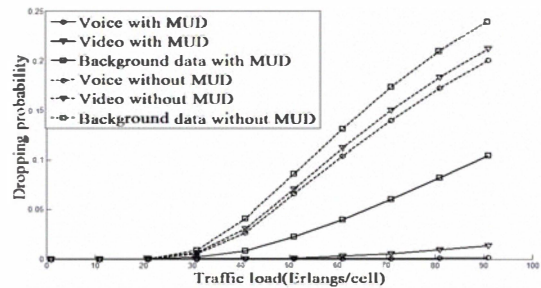
Fig. 8. Averaged dropping probability for different services in IDMA system with and without MUD
