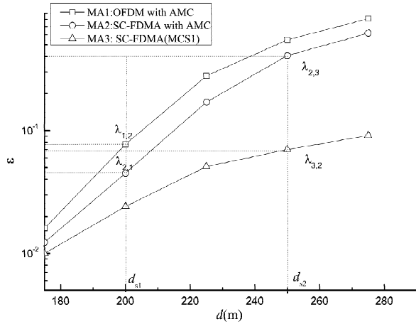
Fig. 4. \varepsilon measurement with different MAs.
