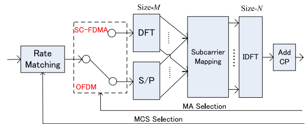
Fig. 1. Diagram of generalized multi-carrier transmitter in the uplink.
