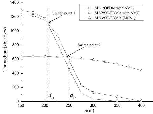
Fig. 3. Throughput comparison between different MAs.
