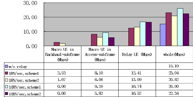
Fig. 8. Comparison of aggregated system throughput
