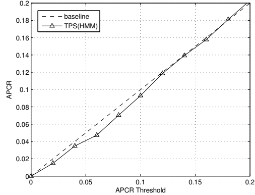
Fig. 6. APCR perceived by the primary user when the idle period of the primary user is hyper-Erlang distribution.
