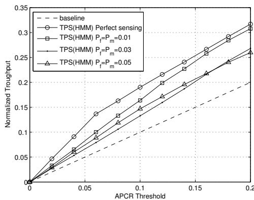
Fig. 10. Normalized throughput of the secondary user with imperfect sensing.
