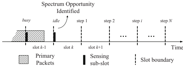
Fig. 3. Spectrum opportunity identification.
