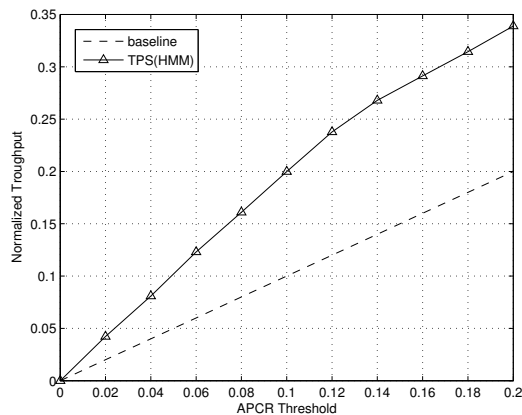
Fig. 8. Normalized throughput of the secondary user when the idle period of the primary user is hyper-Erlang distribution.
