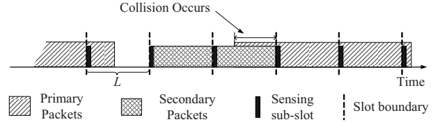
Fig. 2. Slotted structure of the secondary user.
