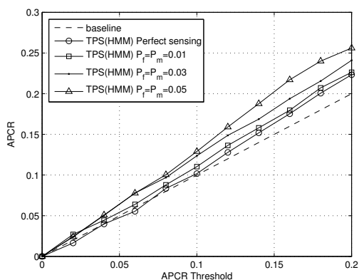
Fig. 9. APCR perceived by the primary user with imperfect sensing.
