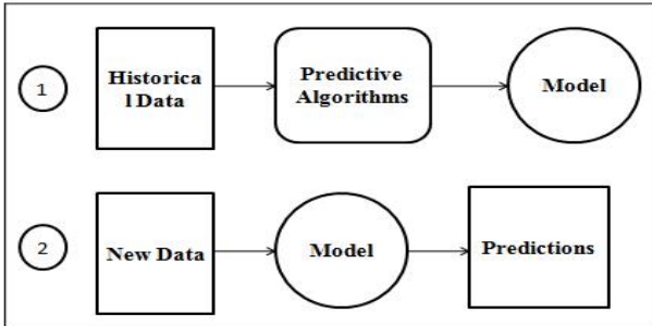
Figure 2. Predictive Analytics
