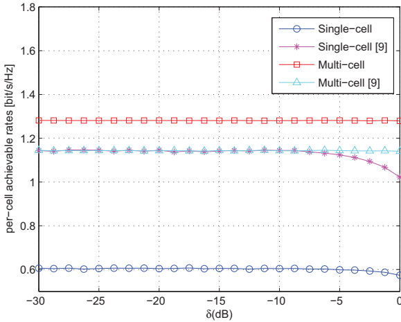
Fig. 6. Ergodic per-cell achievable rates of different schemes for single-cell and multi-cell processing versus the inter-cell gain \delta ( SNR = 5\text{dB} , \beta^2 = -3\text{dB} , d = 0.8 , \sigma = 3 ).
