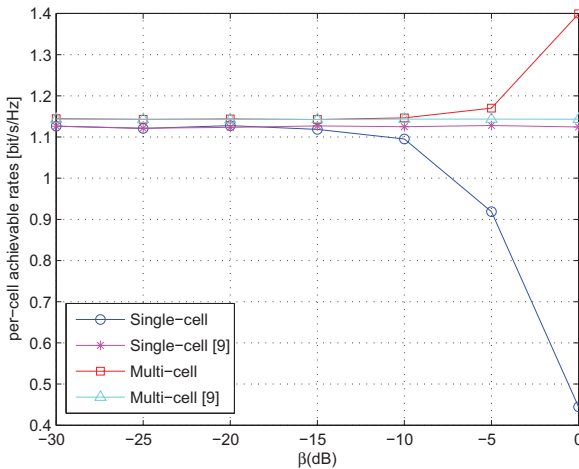
Fig. 7. Ergodic per-cell achievable rates of different schemes for single-cell and multi-cell processing versus the inter-cell gain \beta ( SNR = 5\text{dB} , \delta^2 = -10\text{dB} , d = 0.8 , \sigma = 3 ).
