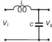
Fig. 2. Passive LC filter circuit (Dewan and Ziogas., 1979).
