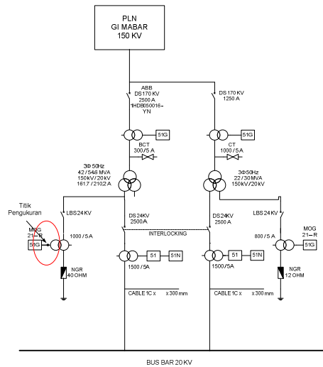
Fig.6. Measurement Point.
