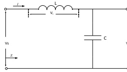
Fig. 3. Passive LC filter impedance circuit.
