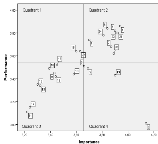
Fig. 2. Cartesian Diagram
