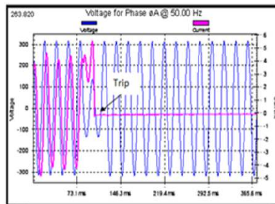
(b) 45% sag magnitude, 100milliseconds sag duration
