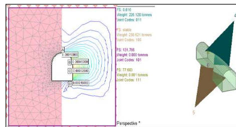
Fig. 3. Total Displacement and Value of Factor Stability Tunnel before Installed Support.
