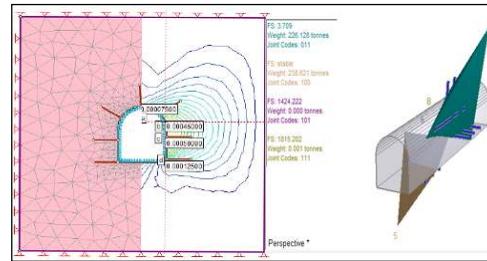
Fig. 4. Total Displacement and Value of Stability Factor for Tunnel after Supporting has been Installed on site.
