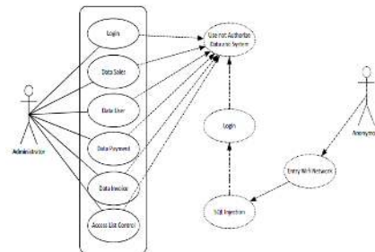
Fig. 2. Miss-Use case.
