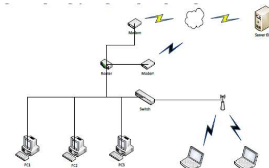
Fig. 1. Network Architecture.
