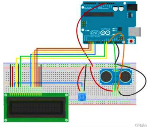
Fig. 9. Arduino Board Wiring, 16x2 LCD, and Ultrasonic Sensor.
