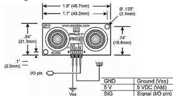
Fig. 1. Ultrasonic Sensor Dimension.
