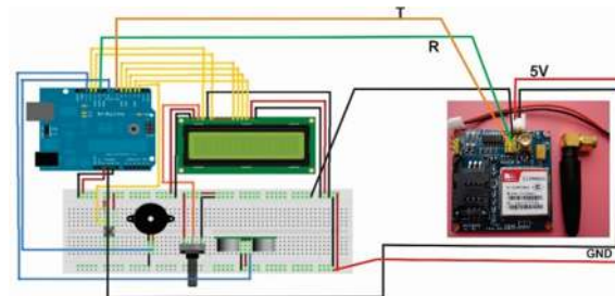
Fig. 11. Wiring with all SIM900A devices and GSM Shield.
