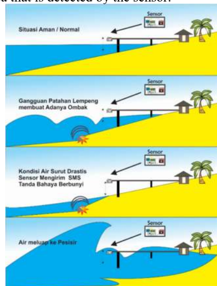
Fig. 16. Prototype Process Works and Tsunami condition.
