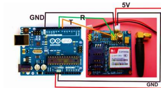
Fig. 8. The Arduino Board and SIM900A.
