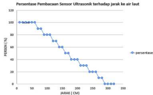
Fig. 15. Graph of percentage ultrasonic sensor readings against distance to sea water.
