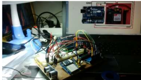
Fig. 12.: Prototype Tsunami Detector.
