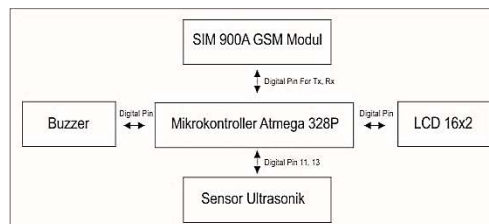
Fig. 13 . Prototype Schematic.
