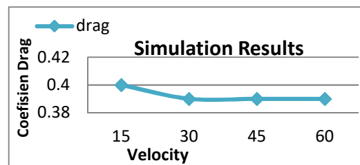
Fig. 8. Graph of Drag Coefficient on Urban Electric Car.
