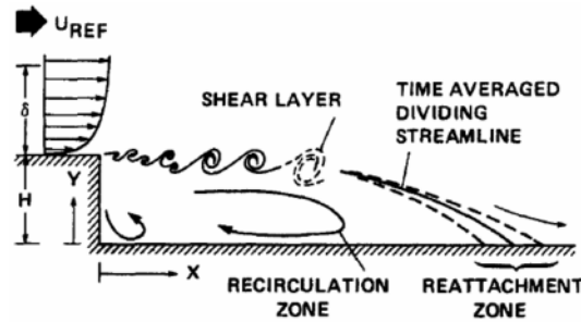
Fig. 3. Schematic of backward-facing step turbulent flow.
