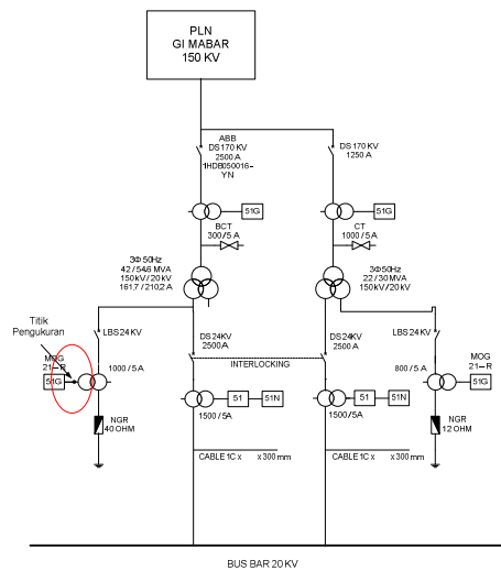
Fig.6. Measurement Point.
