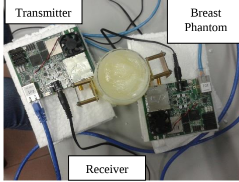
Figure 1: Experimental Set-up
