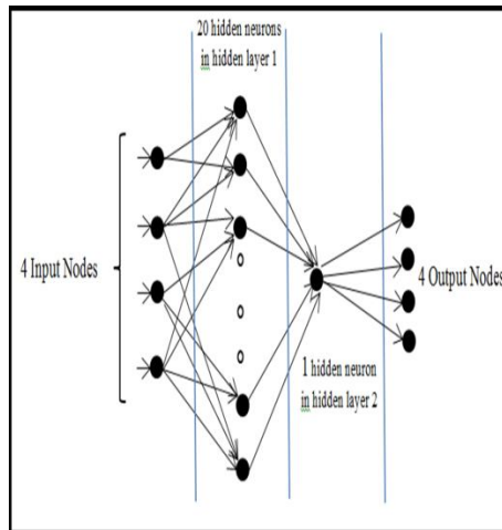
(b) With using Feature Extraction
