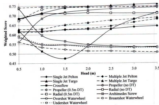
Fig. 5. Weighted for turbine selection to span 13 head 0.5 m to 3.5 m.
