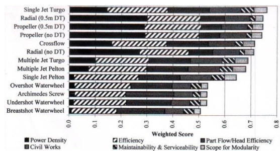
Fig. 6. The value of the score on head 3.5 m for turbine selection with 13 product from each of the different selection criteria.
