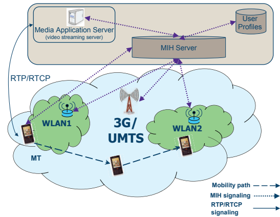
Figure 3: MIH system architecture
