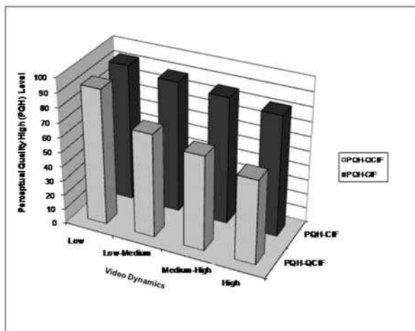
Figure 5: Impact of dynamics on the PQoS saturation point
