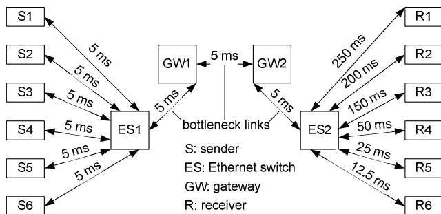
Figure 17. Network topology used to evaluate fairness and friendliness.
