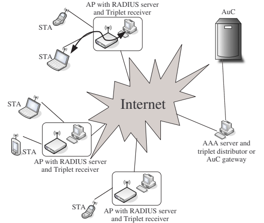
Figure 5: Architecture for our modified EAP-SIM authentication
