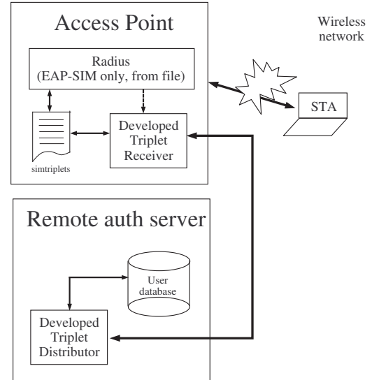
Figure 6: System model
