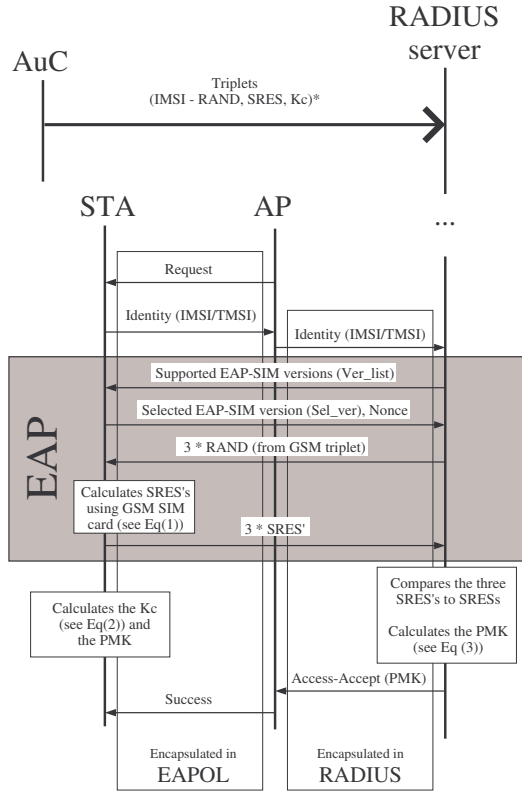
Figure 4: Process of EAP-SIM authentication
