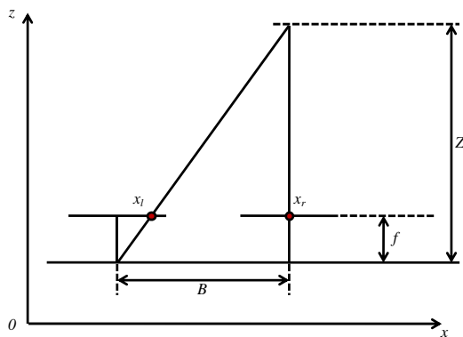
Figure 4. Relationship between disparity and depth
