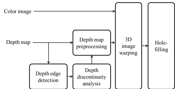
Figure 6. Block diagram of the proposed scheme
