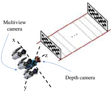
Figure 3. Depth calibration
