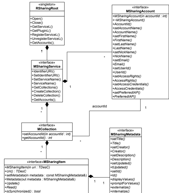
Figure 5. Relations between sharing root, services and items
