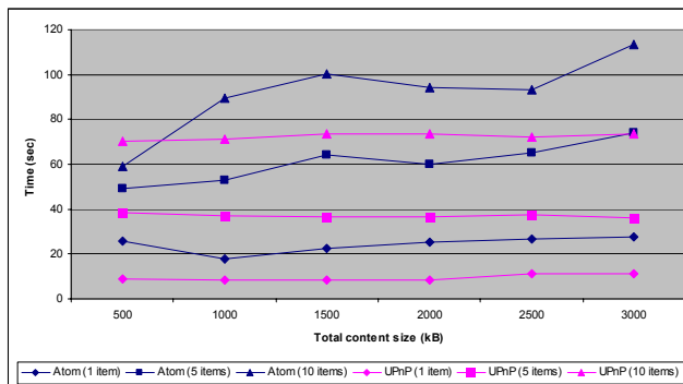
Figure 8. Total upload times, using Atom & UPnP
