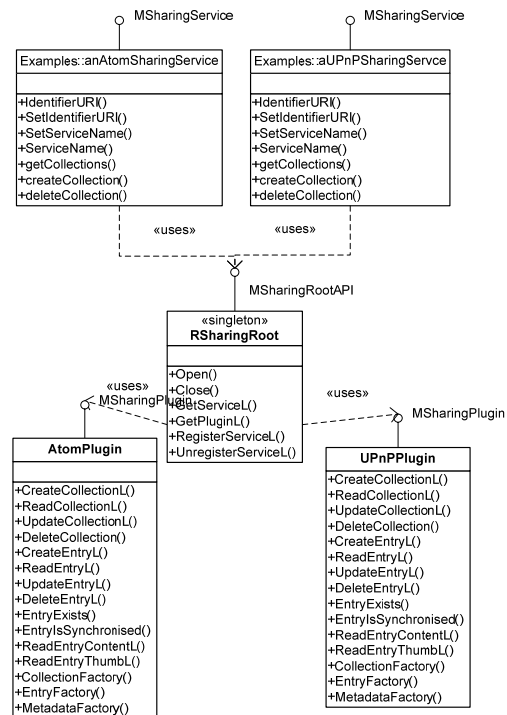
Figure 3. Relations of sharing root, services and plug-ins
