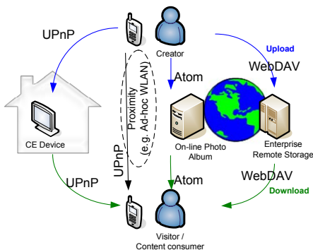
Figure 1. Example of content sharing protocols
