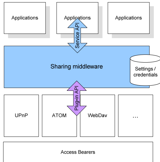
Figure 2. Sharing Middleware Simplified Design
