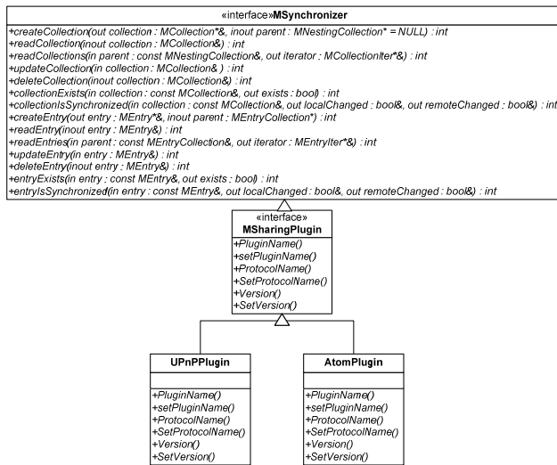
Figure 4. MSharingPlugin and derived classes
