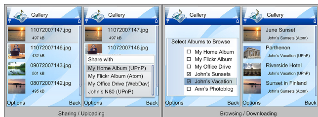
Figure 7. Concept UI for uploading & downloading content
