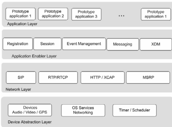
Figure 3. Client Service Creation Environment
